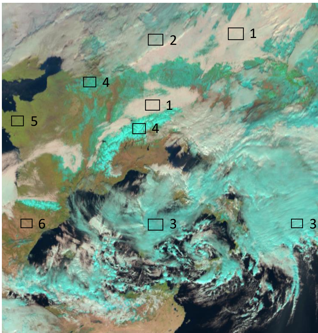
SEVIRI Natural Colour RGB, 18 January 2017, 12:00 UTC
