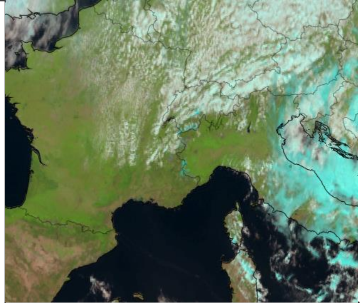
SEVIRI Natural Colour RGB, 15 July 2016, 12:00 UTC
