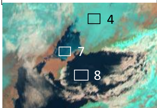
Natural Colour RGB, 17 February 2017, 12:00 UTC
